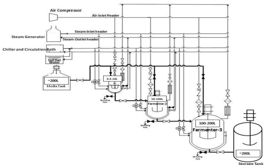
Fermentation Setup Flowchart Diagram
